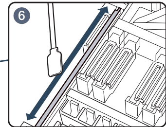
6 Clean wiper rail(s).
