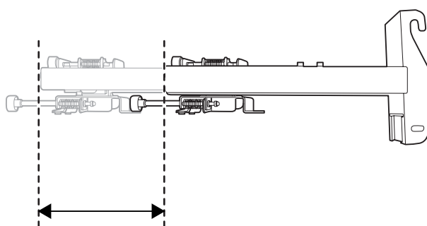
Forward/backward slide adjustment range: 0 to 11.81 in. (300 mm)
