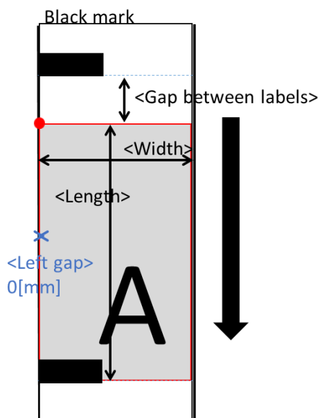
Figure 4.3.2-5 Wristband layout
