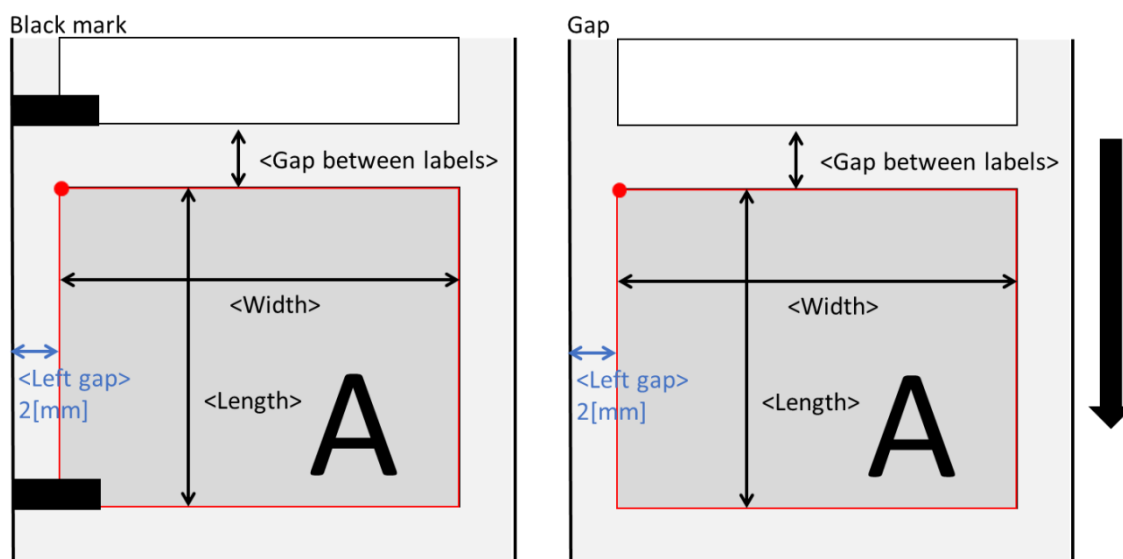
Figure 4.3.2-2 Die-cut label layout
