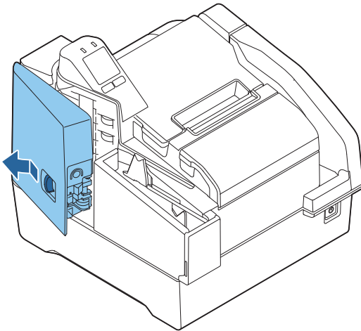
<Scanner cover>
